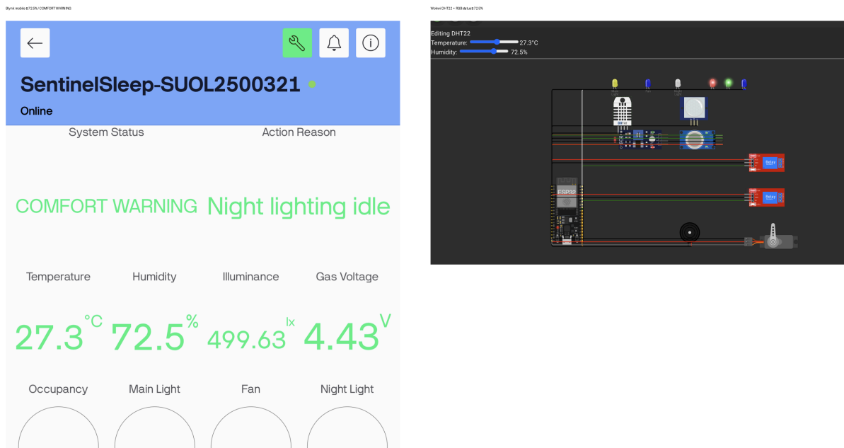
Figure 6. Live Blynk mobile and Wokwi humidity-warning evidence. The mobile dashboard reports 72.5% humidity and COMFORT WARNING ; the matching Wokwi DHT22 control and red-plus-green RGB warning indicators are shown beside it. Source: Author's implementation.
